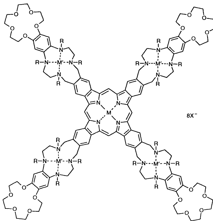
Scheme 1 ts = Tosyl ( p -MeC 6 H 4 SO 2 ). (i) dmf, K 2 CO 3 ; (ii) tosyl chloride, pyridine; (iii) dmf, K 2 CO 3 , 1,2-dibromo-4,5-bis(bromomethyl)benzene; (iv) dmf, CuCN; (v) pyridine, CuCN; (vi) dmf, NiCl 2 ; (vii) quinoline, CuCN
